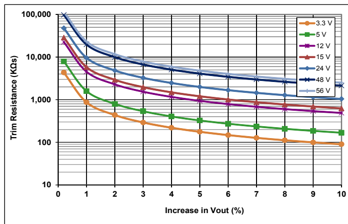
Common Figure 3: Trim graph for trim-up 3.3V to 56V outputs.
