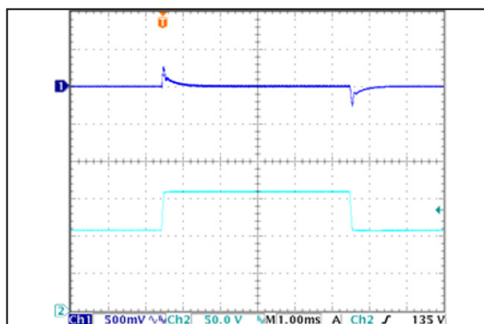
Figure 6: Output voltage response to step-change in input voltage (1V/ \mu\text{s} ). Load cap: 1 \mu\text{F} ceramic and 15 \mu\text{F} tantalum capacitors. Ch 1: V_{out} , Ch 2: V_{in} .
